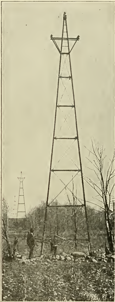
Fig. 174. Steel Tower with only Side Bracing
